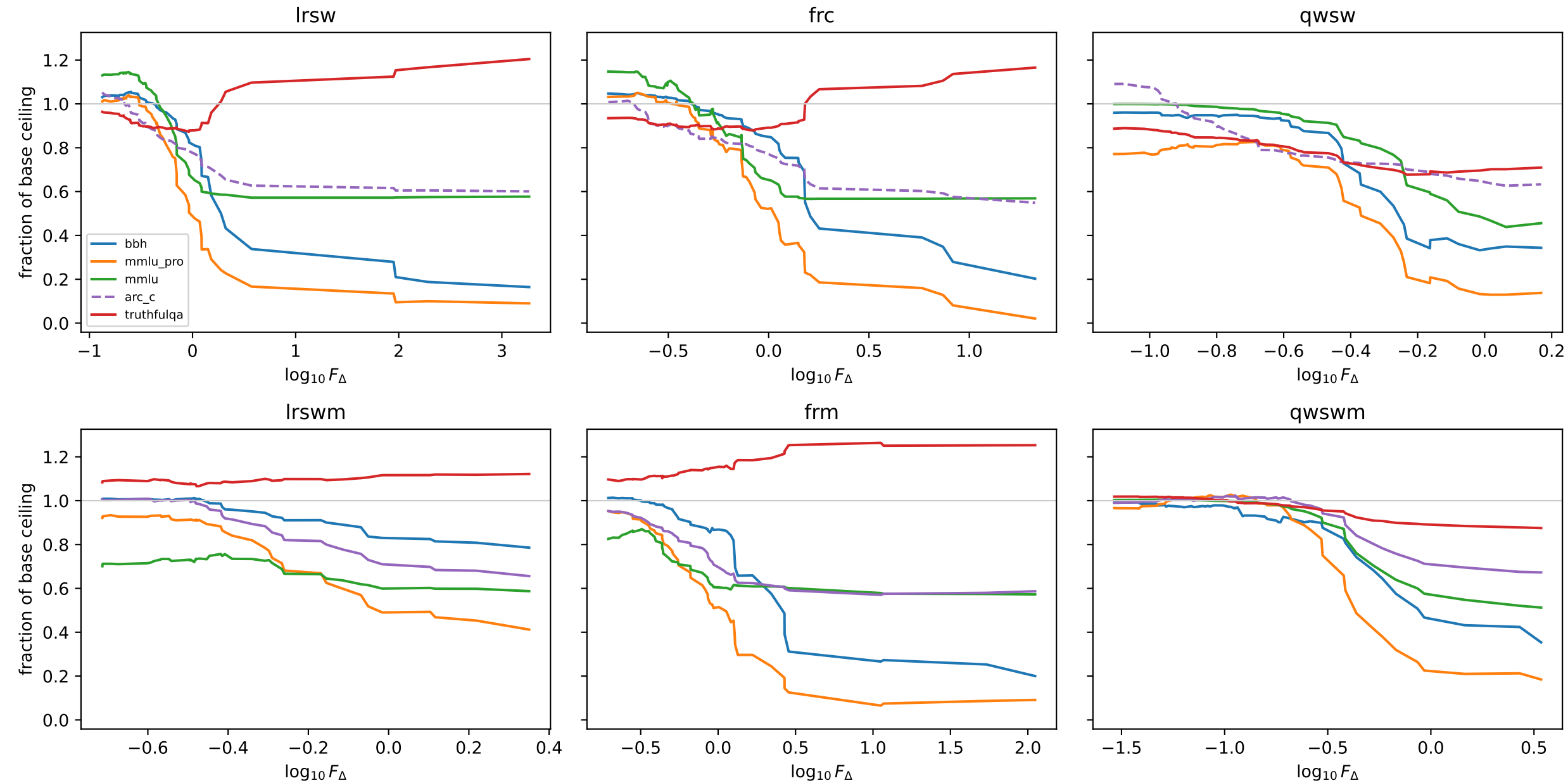
Per-benchmark degradation (rolling mean over cells; dashed = trained-on/contaminated)
